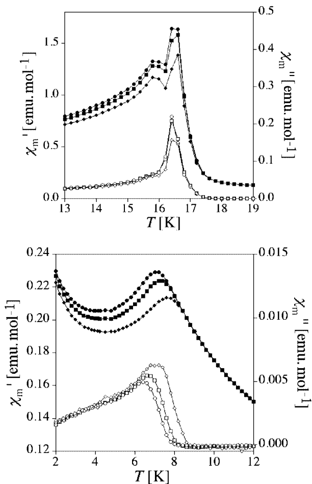
Figure 5. Frequency dependence of the in-phase (filled symbols, \chi'_m ) and out-of-phase (empty symbols, \chi''_m ) AC magnetic susceptibility for the salts [\text{Ru}(\text{bpy})_3][\text{ClO}_4][\text{M}^{\text{II}}(\text{ox})_3] at 1 (circle), 10 (square) and 332 Hz (diamond); \text{M}^{\text{II}} = \text{Mn} (top), \text{Fe} (bottom).
