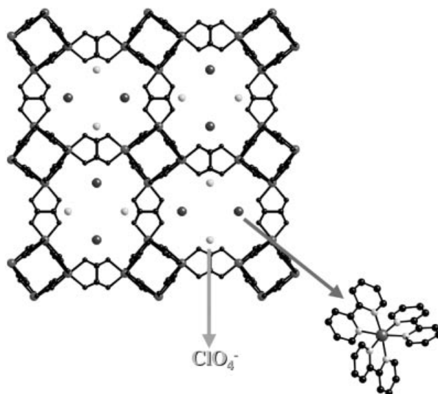
Figure 1. Projection on the bc plane of the structure of the family of molecule-based magnets [Z^{II}(\text{bpy})_3][\text{ClO}_4][\text{M}^{II}\text{M}^{III}(\text{ox})_3] . Only the Z^{II} ion of the [Z^{II}(\text{bpy})_3]^{2+} cations and the Cl atom of the \text{ClO}_4^- anions are drawn in the cavities.
