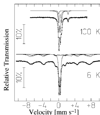
Figure 6. Mössbauer spectra at different temperatures for the salt [\text{Fe}(\text{bpy})_3][\text{ClO}_4][\text{MnFe}(\text{ox})_3] .
